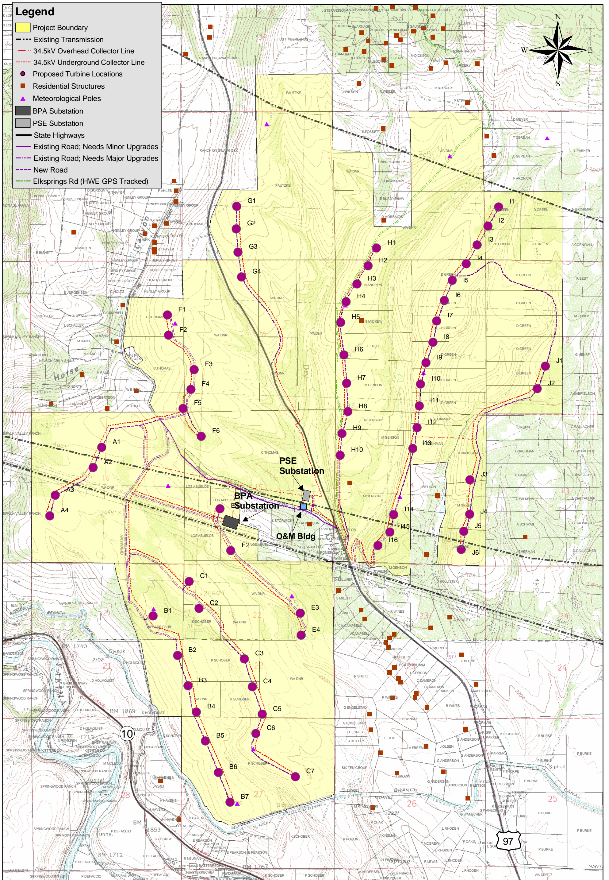
EIS Figure 2-1: Kittitas Valley Wind Power Project Site Layout Source: Schafer 2005i
