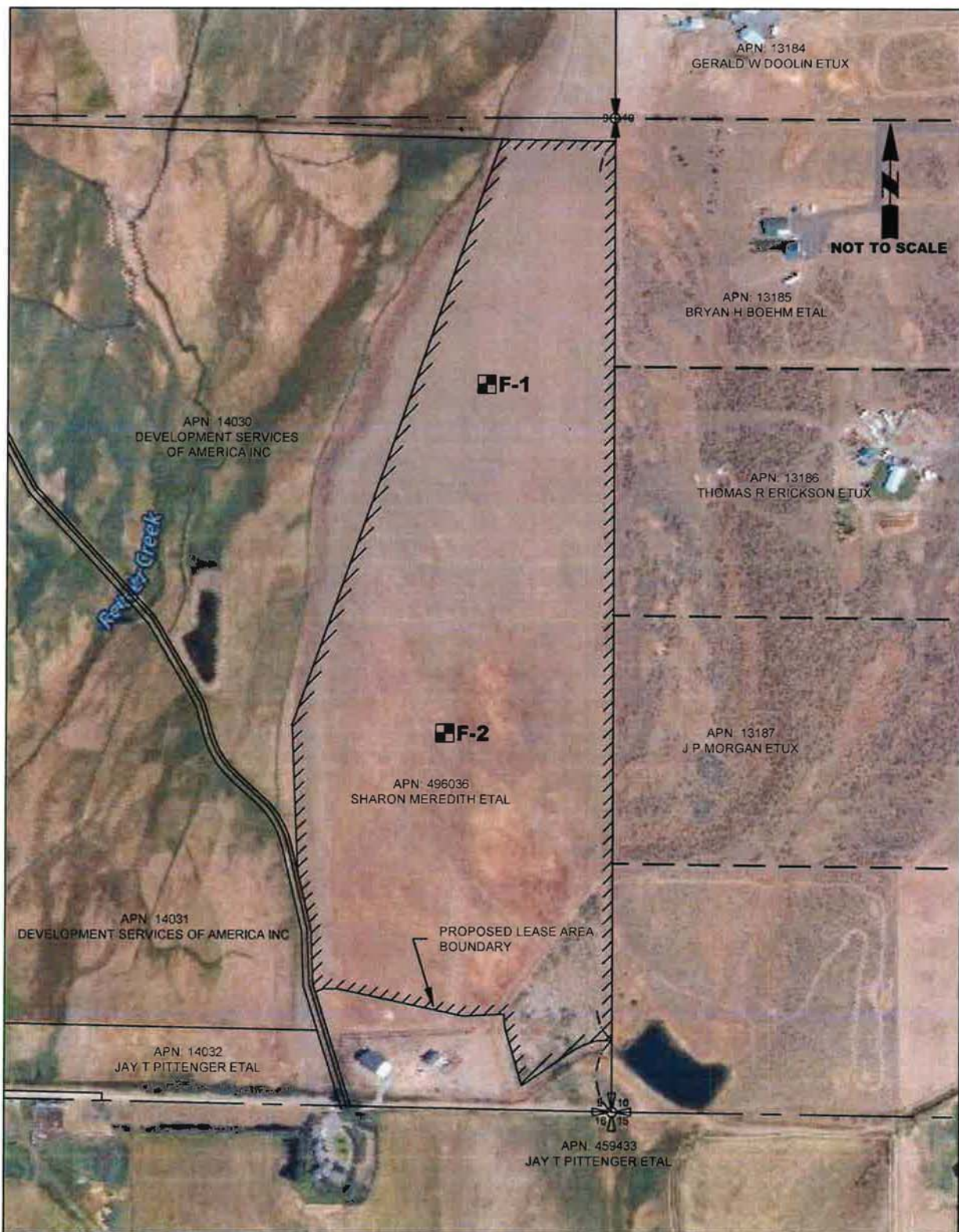
FIG. 2 FUMARIA SITE TEST BORING LOCATIONS
