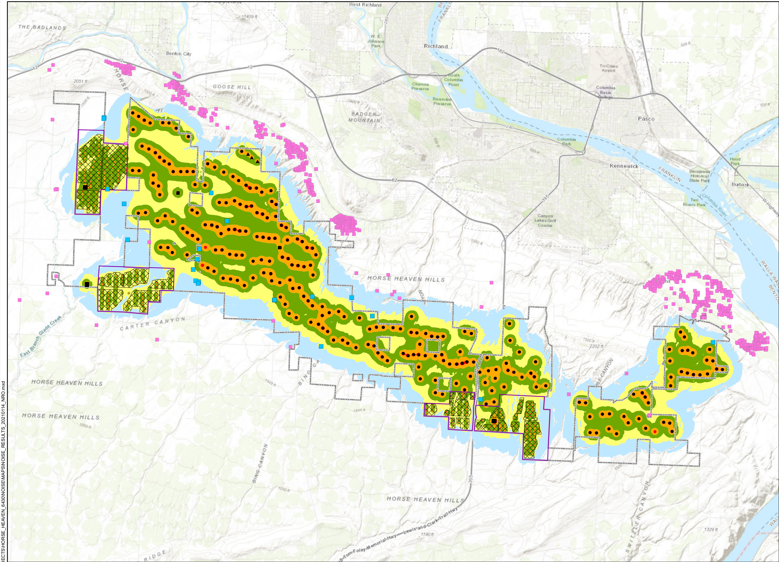
Figure 4.1.1-2 Operational Received Sound Levels Option 1 G.E. 2.82 MW Wind Turbines (NRO Mode) BENTON COUNTY, WA
