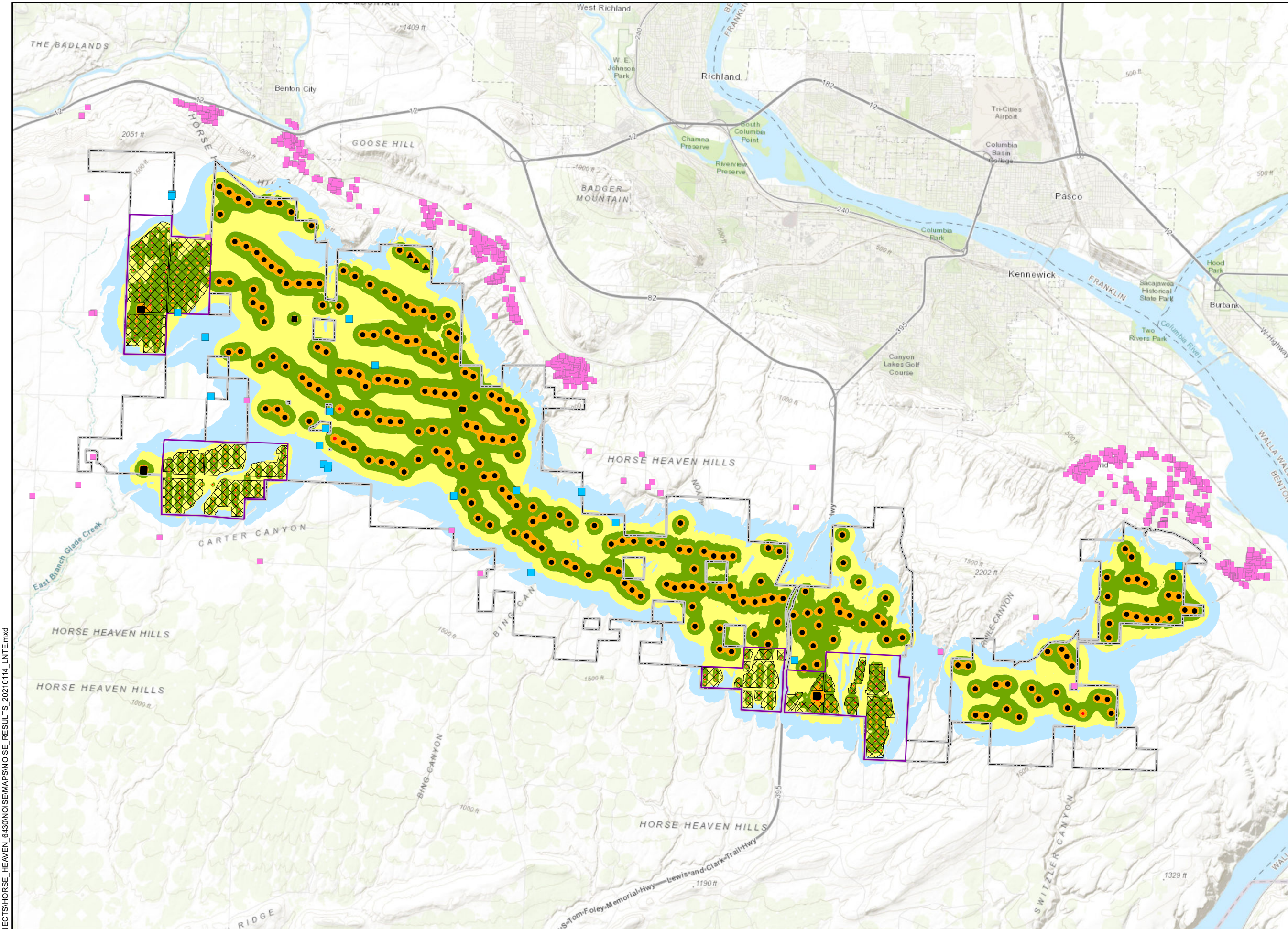
Figure 4.1.1-3 Operational Received Sound Levels Option 1 G.E. 3.03 MW Wind Turbines (LNTE) BENTON COUNTY, WA
