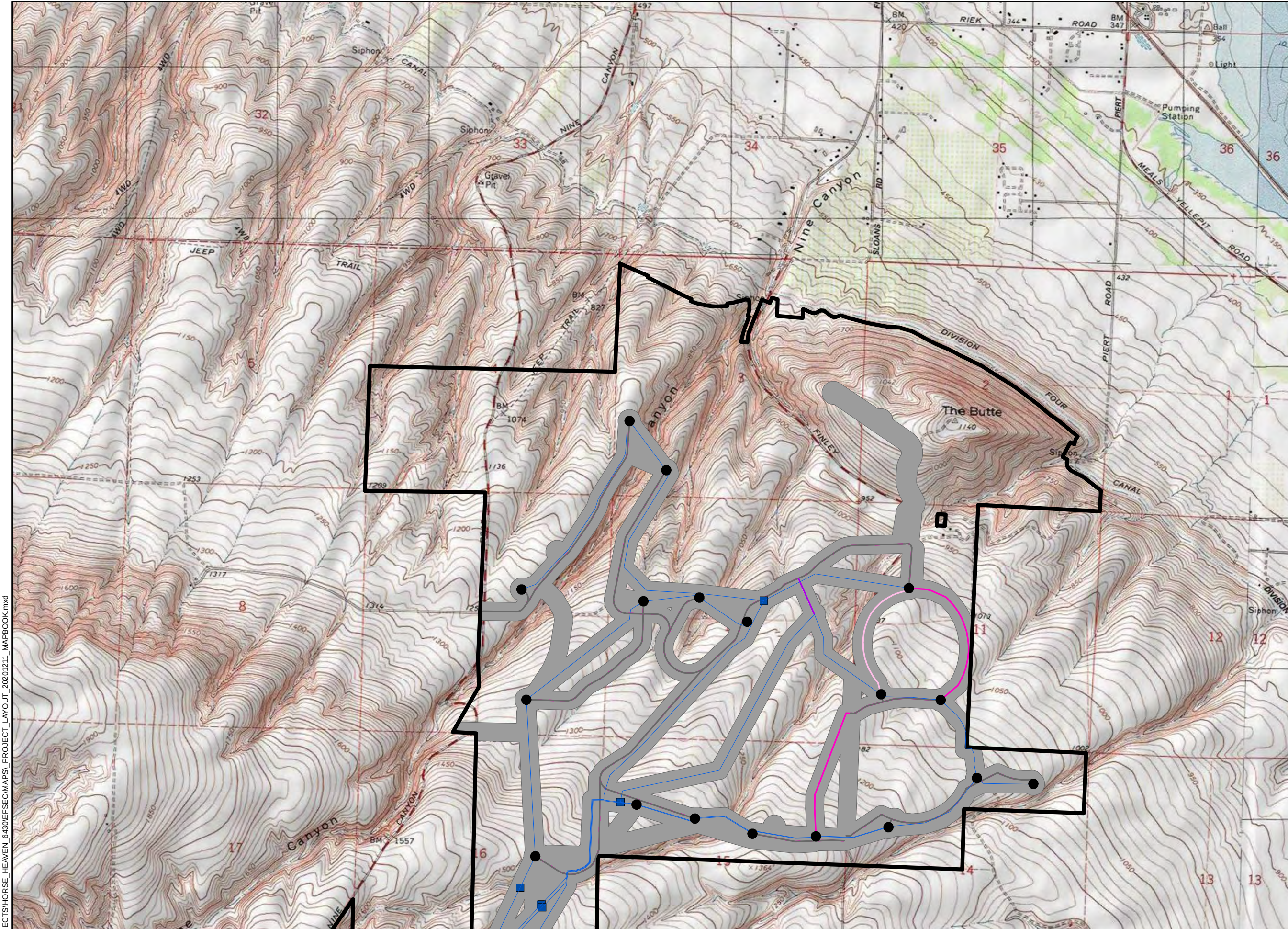
Figure 2 Facility Infrastructure for Turbine Layout Option 1 Map 11 of 11 BENTON COUNTY, WA
